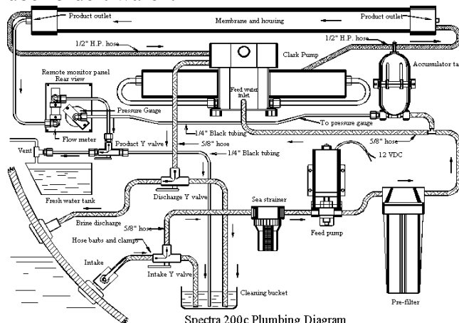
Spectra 200c Plumbing Diagram
